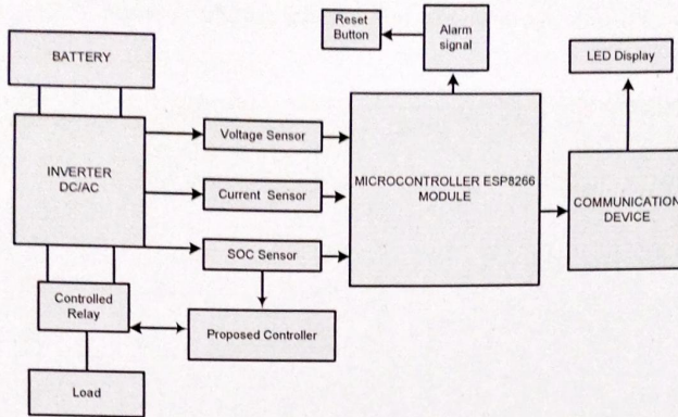
Fig.1. Block Diagram of integrated SMART INVERTER
